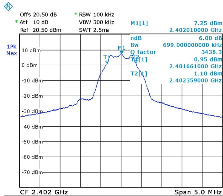
Figure 16. 2402.0 MHz
