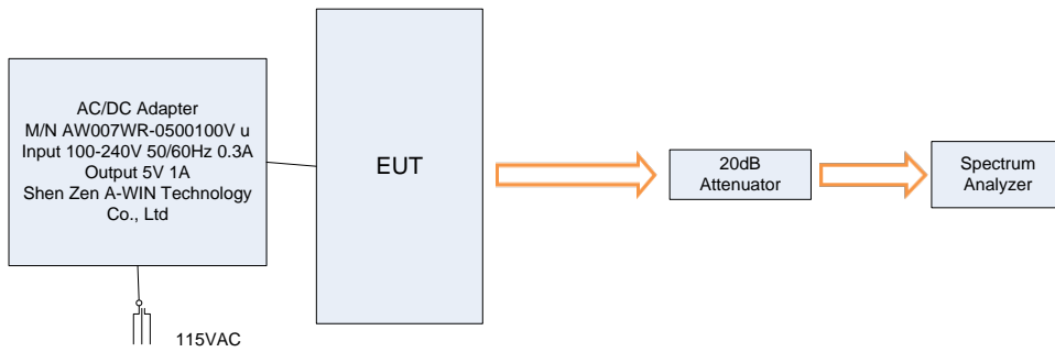
Figure 2. Configuration of Tested System Conducted
