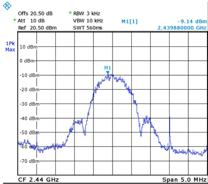
Figure 39 — 2440.0 MHz
